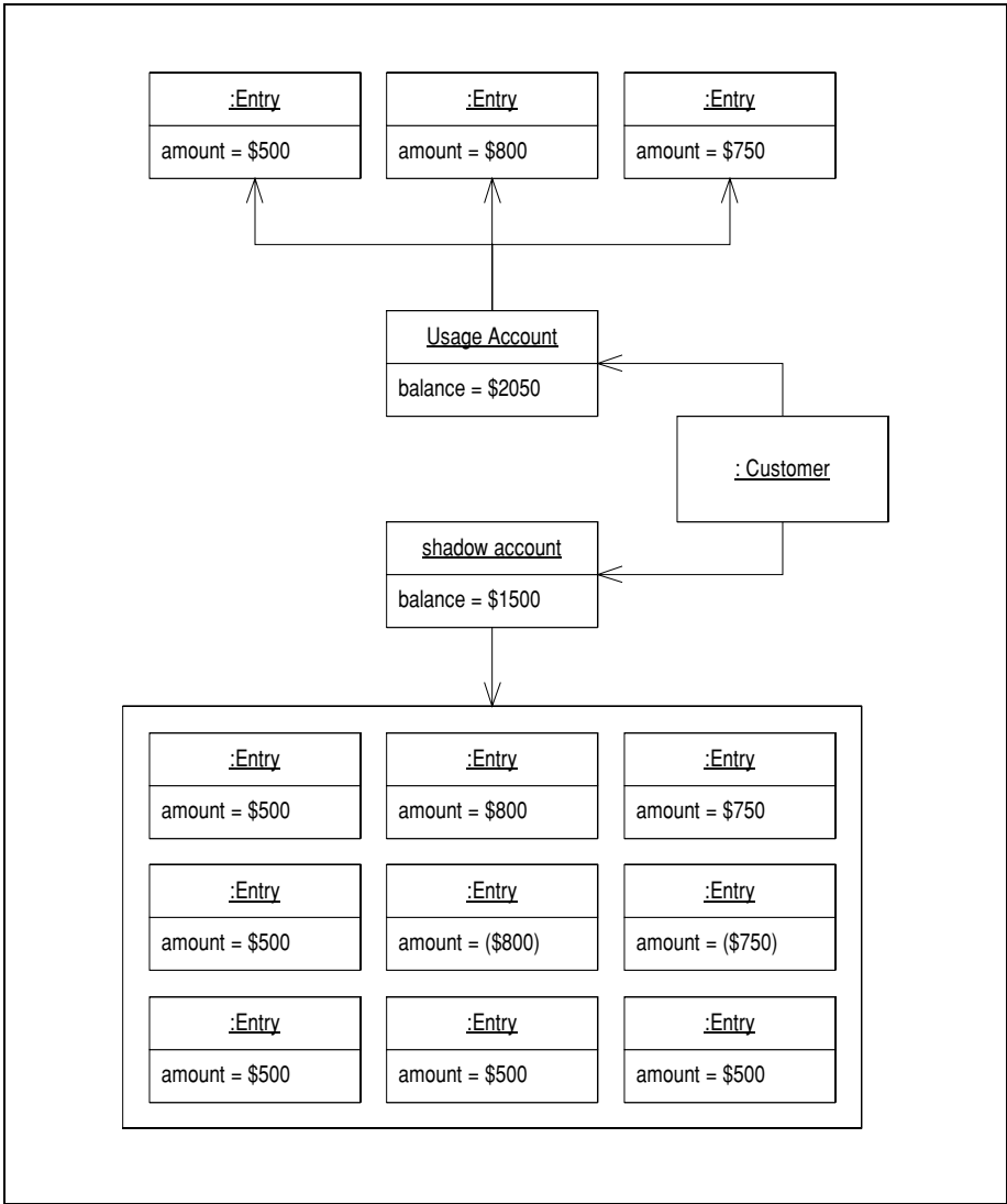
Figure 0.28 After posting the reversals and new entries.
