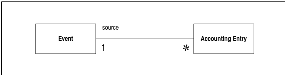
Figure 0.8 Keeping a link between an event and its resulting entries
