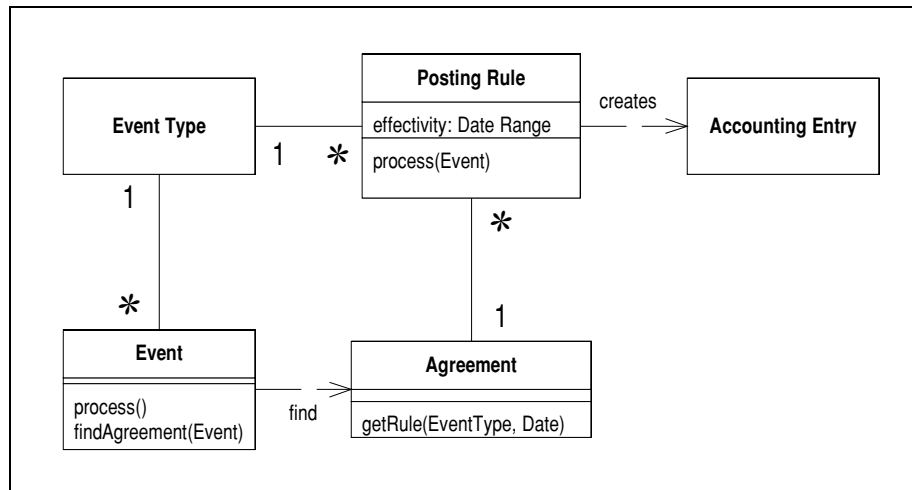
Figure 0.5 Allowing rules to vary by date.
